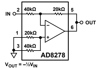
Figure 55. Inverting Amplifier, Gain = -1/2
