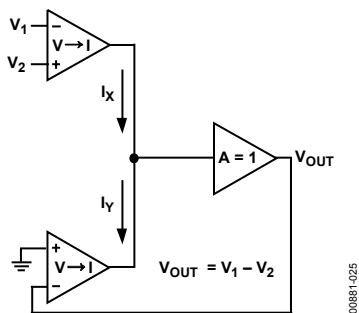
Figure 25. AD830 as a Difference Amplifier
