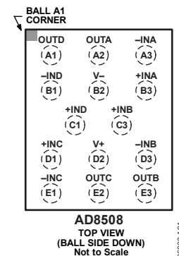
Figure 6. 14-Ball WLCSP (CB-14-1)
