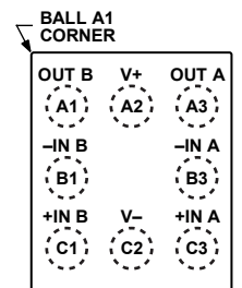
Figure 2. 6-Ball WLCSP (CB-6-7)
