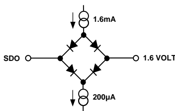
Figure 3. AC Timing SDO Pin Load Circuit
