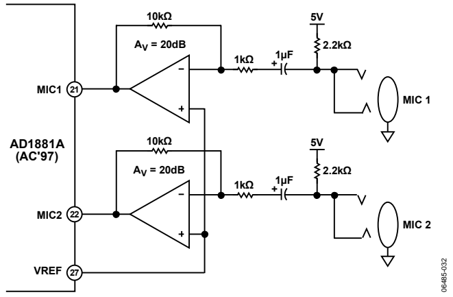
Figure 32. Microphone Preamplifier
