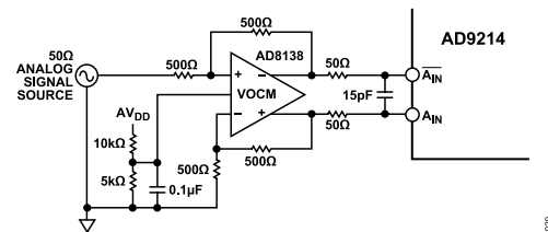
Figure 29. DC-Coupled Analog Input Circuit
