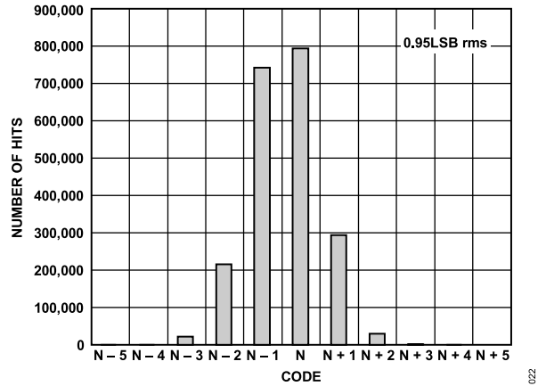
Figure 24. Input Referred Noise Histogram; f_{SAMPLE} = 80 \text{ MSPS}
