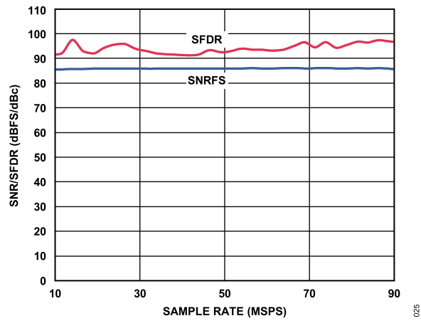
Figure 27. SNR/SFDR vs. Sample Rate; f_{IN} = 70 MHz, f_{SAMPLE} = 80 MSPS
