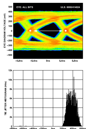
Figure 69. Data Eye for LVDS Outputs in ANSI-644 Mode with Trace Lengths Greater Than 24 Inches on Standard FR-4 Material, External 100 Ω Far-End Termination Only
