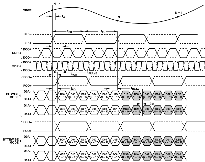
Figure 3. 12-Bit DDR/SDR, Two-Lane, 1x Frame Mode
