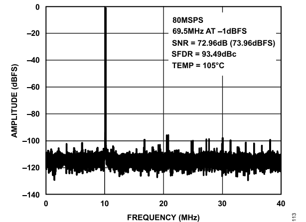
Figure 13. Single-Tone 16k FFT with f_{IN} = 69.5 MHz, f_{SAMPLE} = 80 MSPS, Temp = 105°C
