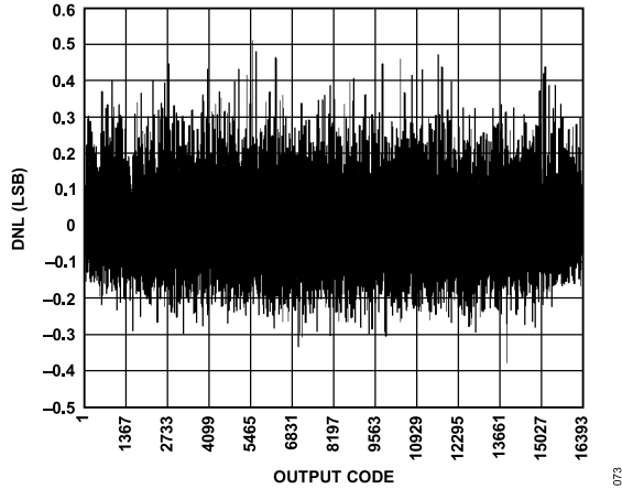
Figure 40. DNL; f_{IN} = 9.7 \text{ MHz} , f_{SAMPLE} = 125 \text{ MSPS}
