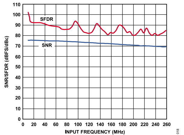
Figure 20. SNR/SFDR vs. f_{IN} ; f_{SAMPLE} = 80 MSPS
