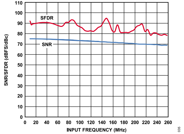
Figure 37. SNR/SFDR vs. f_{IN} ; f_{SAMPLE} = 125 \text{ MSPS}
