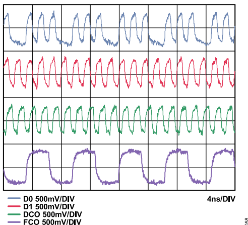
Figure 66. AD9645-125, LVDS Output Timing Example in ANSI-644 Mode (Default)
