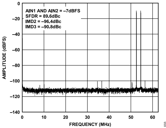
Figure 35. Two-Tone 16k FFT with f_{IN1} = 70.5 \text{ MHz} and f_{IN2} = 72.5 \text{ MHz} , f_{SAMPLE} = 125 \text{ MSPS}
