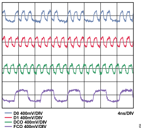
Figure 67. AD9645-125, LVDS Output Timing Example in Reduced Range Mode
