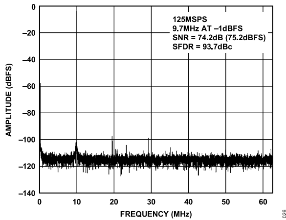
Figure 28. Single-Tone 16k FFT with f_{IN} = 9.7 MHz, f_{SAMPLE} = 125 MSPS
