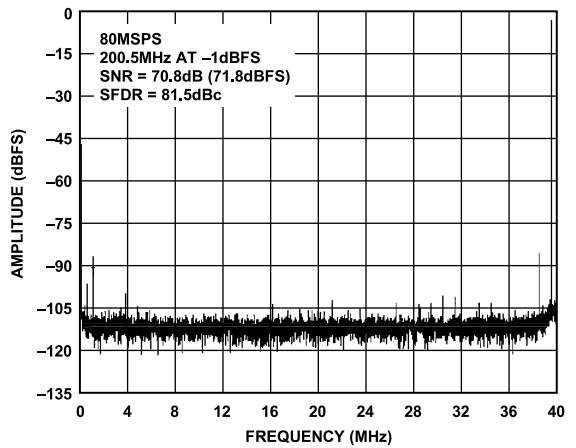
Figure 16. Single-Tone 16k FFT with f_{IN} = 200.5 MHz, f_{SAMPLE} = 80 MSPS, Clock Divide = Divide-by-8
