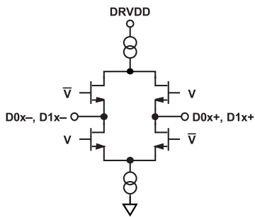
Figure 48. Equivalent Digital Output Circuit
