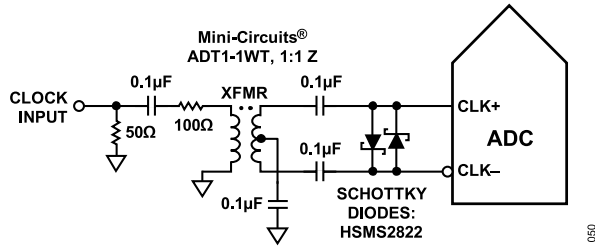
Figure 59. Transformer-Coupled Differential Clock (Up to 200 MHz)
