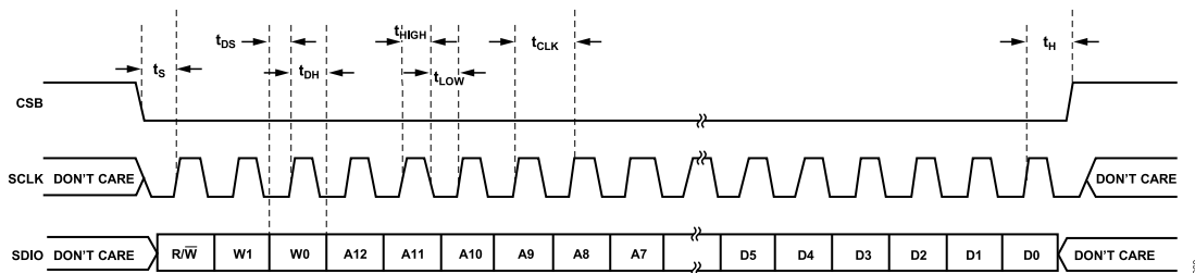
Figure 70. Serial Port Interface Timing Diagram
