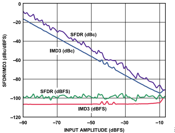
Figure 36. Two-Tone SFDR/IMD3 vs. Input Amplitude (AIN) with f_{IN1} = 70.5 \text{ MHz} and f_{IN2} = 72.5 \text{ MHz} , f_{SAMPLE} = 125 \text{ MSPS}
