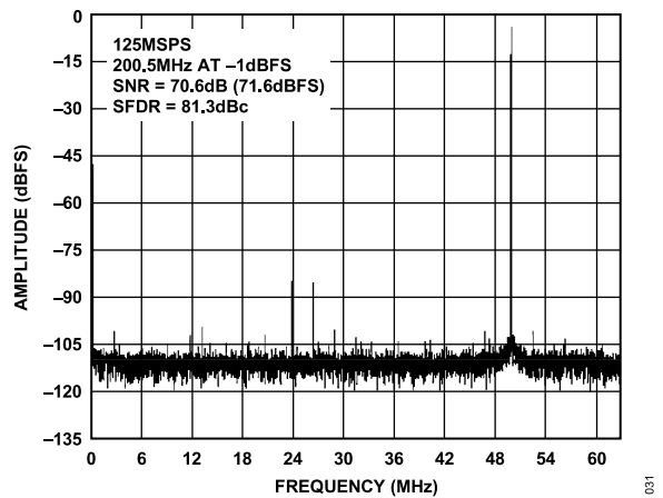
Figure 33. Single-Tone 16k FFT with f_{IN} = 200.5 MHz, f_{SAMPLE} = 125 MSPS, Clock Divide = Divide-by-8
