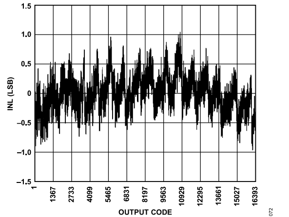
Figure 39. INL; f_{IN} = 9.7 \text{ MHz} , f_{SAMPLE} = 125 \text{ MSPS}
