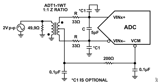
Figure 56. Differential Transformer-Coupled Configuration for Baseband Applications
