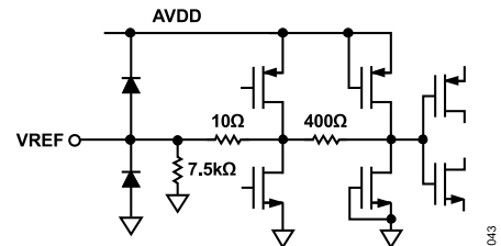
Figure 52. Equivalent VREF Circuit
