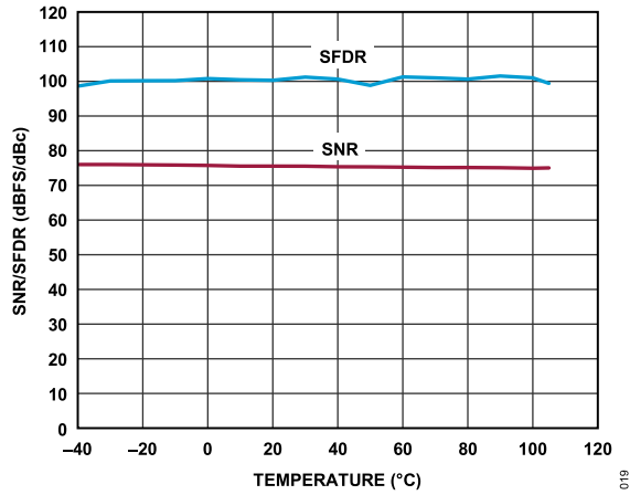
Figure 21. SNR/SFDR vs. Temperature; f_{IN} = 9.7 \text{ MHz} , f_{SAMPLE} = 80 \text{ MSPS}
