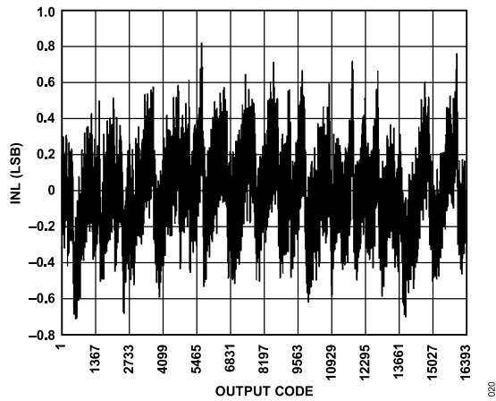
Figure 22. INL; f_{IN} = 9.7 \text{ MHz} , f_{SAMPLE} = 80 \text{ MSPS}
