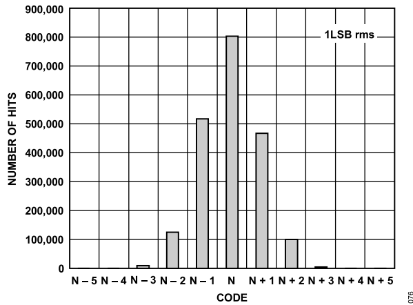
Figure 41. Input Referred Noise Histogram; f_{SAMPLE} = 125 \text{ MSPS}
