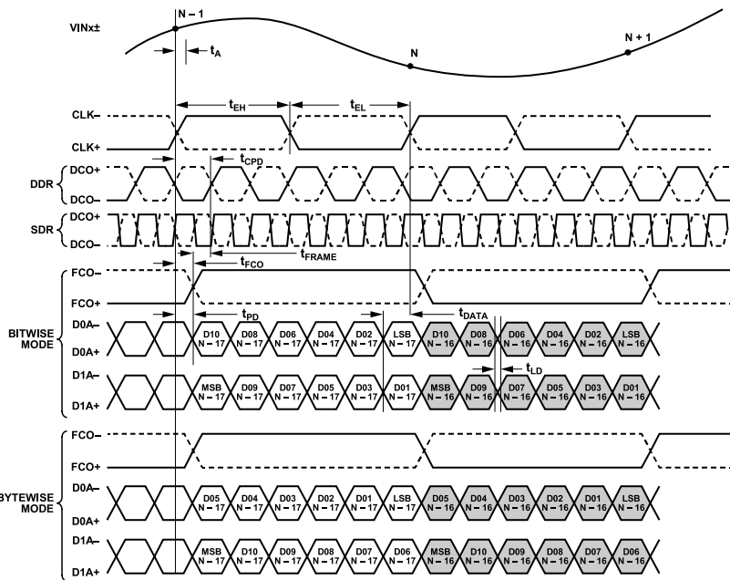
Figure 5. 12-Bit DDR/SDR, Two-Lane, 2x Frame Mode
