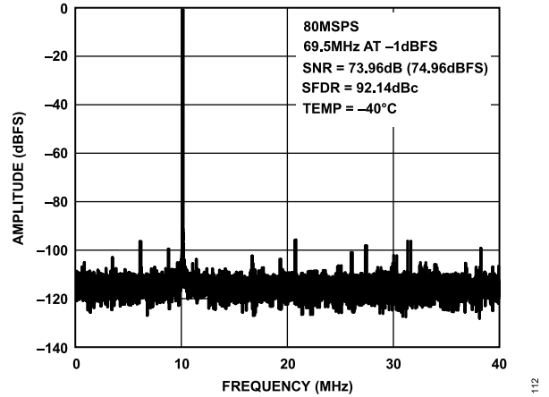
Figure 12. Single-Tone 16k FFT with f_{IN} = 69.5 MHz, f_{SAMPLE} = 80 MSPS, Temp = -40°C
