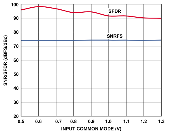
Figure 54. SNR/SFDR vs. Input Common-Mode Voltage, f_{IN} = 9.7 MHz, f_{SAMPLE} = 125 MSPS
