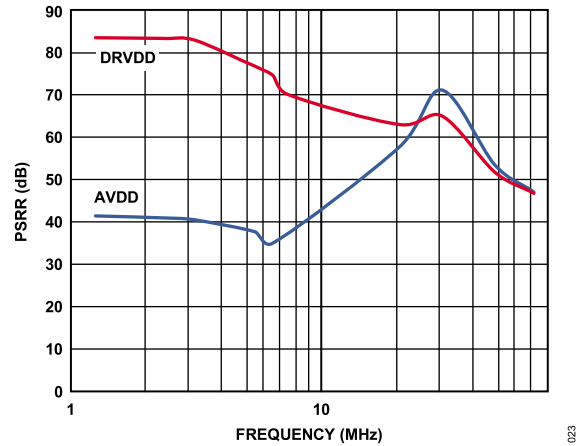
Figure 25. PSRR vs. Frequency; f_{CLK} = 125 \text{ MHz} , f_{SAMPLE} = 80 \text{ MSPS}
