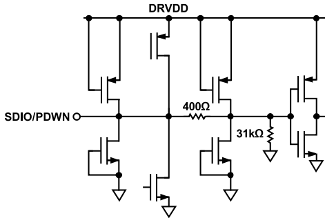
Figure 47. Equivalent SDIO/PDWN Input Circuit
