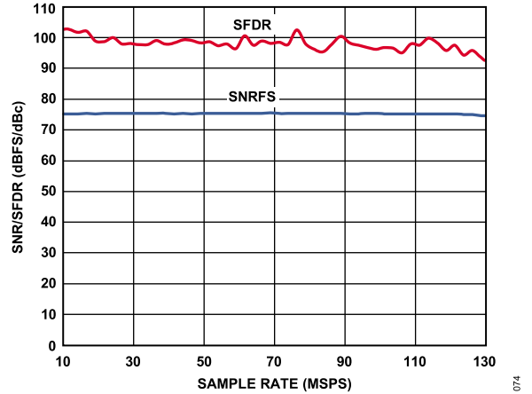
Figure 43. SNR/SFDR vs. Sample Rate; f_{IN} = 9.7 \text{ MHz} , f_{SAMPLE} = 125 \text{ MSPS}
