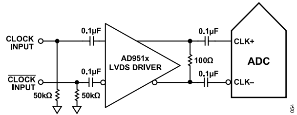
Figure 62. Differential LVDS Sample Clock (Up to 1 GHz)
