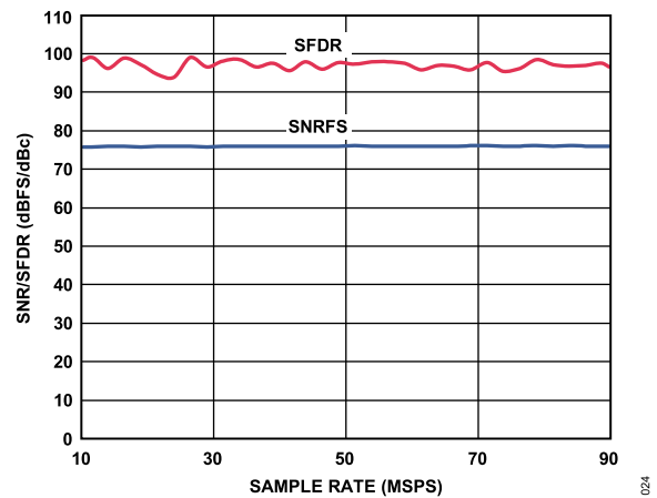
Figure 26. SNR/SFDR vs. Sample Rate; f_{IN} = 9.7 \text{ MHz} , f_{SAMPLE} = 80 \text{ MSPS}
