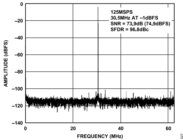
Figure 29. Single-Tone 16k FFT with f_{IN} = 30.5 MHz, f_{SAMPLE} = 125 MSPS
