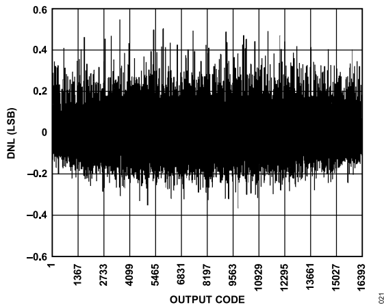
Figure 23. DNL; f_{IN} = 9.7 \text{ MHz} , f_{SAMPLE} = 80 \text{ MSPS}
