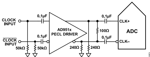
Figure 61. Differential PECL Sample Clock (Up to 1 GHz)
