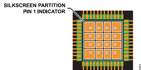
Figure 71. Typical PCB Layout
