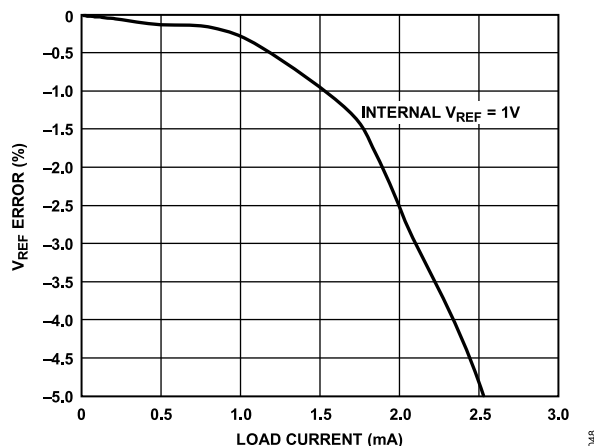
Figure 57. V_{REF} Error vs. Load Current
