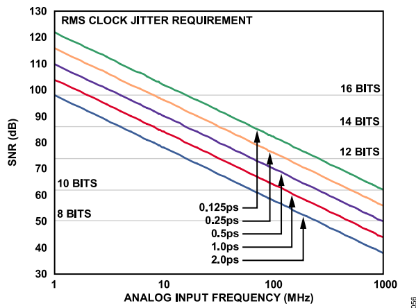
Figure 64. Ideal SNR vs. Input Frequency and Jitter
