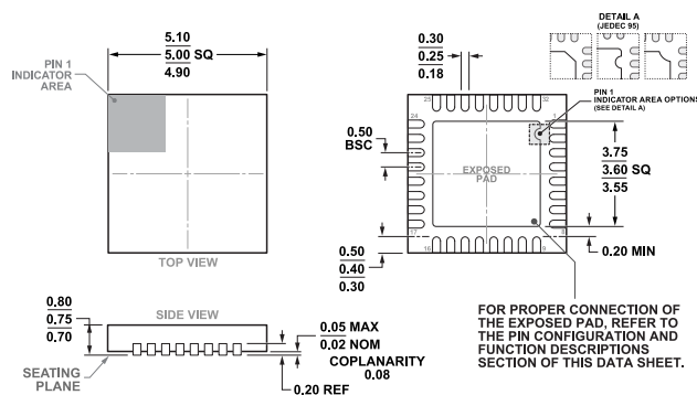
Figure 72. 32-Lead Lead Frame Chip Scale Package [LFCSP] 5 mm x 5 mm Body and 0.75 mm Package Height (CP-32-12)
