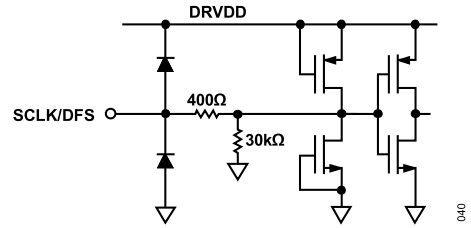
Figure 49. Equivalent SCLK/DFS Input Circuit
