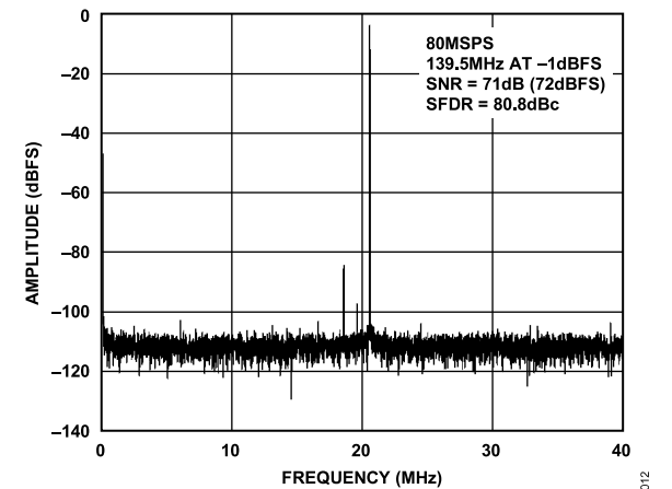
Figure 14. Single-Tone 16k FFT with f_{IN} = 139.5 MHz, f_{SAMPLE} = 80 MSPS
