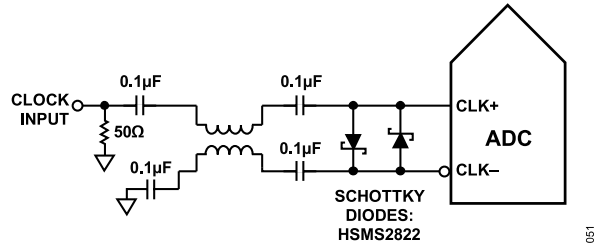
Figure 60. Balun-Coupled Differential Clock (Up to 1 GHz)
