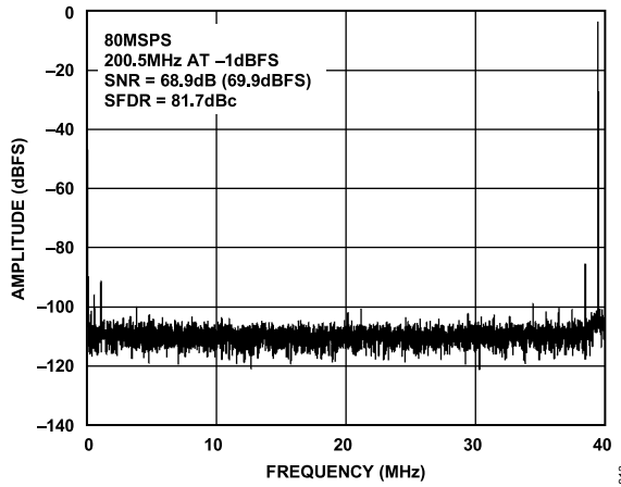
Figure 15. Single-Tone 16k FFT with f_{IN} = 200.5 MHz, f_{SAMPLE} = 80 MSPS
