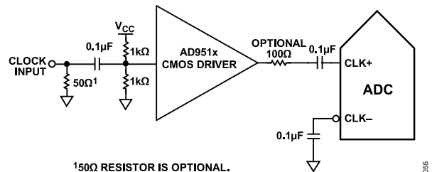
Figure 63. Single-Ended 1.8 V CMOS Input Clock (Up to 200 MHz)
