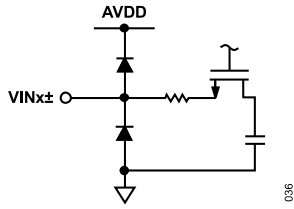
Figure 45. Equivalent Analog Input Circuit
