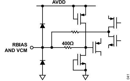
Figure 50. Equivalent RBIAS and VCM Circuit
