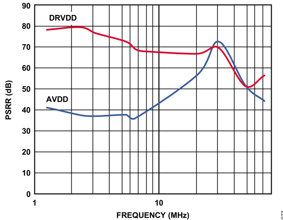
Figure 42. PSRR vs. Frequency; f_{CLK} = 125 \text{ MHz} , f_{SAMPLE} = 125 \text{ MSPS}
