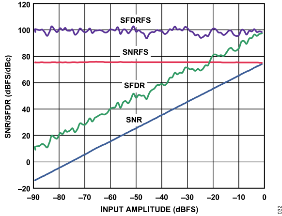
Figure 34. SNR/SFDR vs. Analog Input Level; f_{IN} = 9.7 \text{ MHz} , f_{SAMPLE} = 125 \text{ MSPS}
