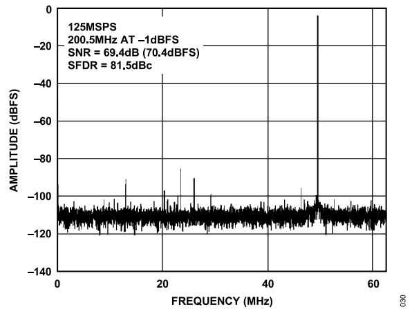
Figure 32. Single-Tone 16k FFT with f_{IN} = 200.5 MHz, f_{SAMPLE} = 125 MSPS
