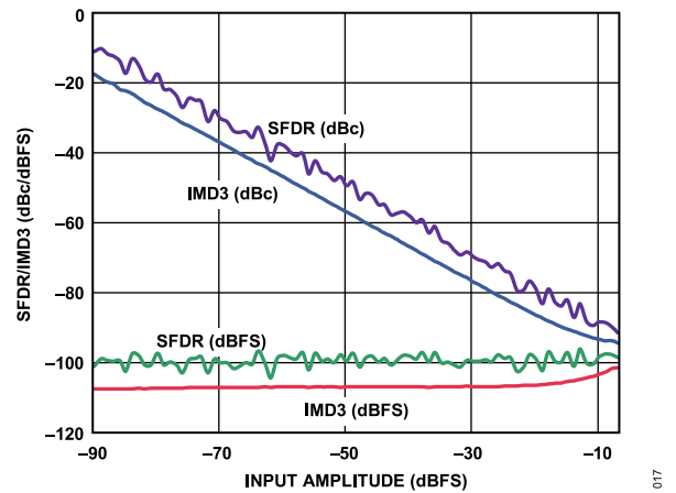
Figure 19. Two-Tone SFDR/IMD3 vs. Input Amplitude (AIN) with f_{IN1} = 70.5 MHz and f_{IN2} = 72.5 MHz, f_{SAMPLE} = 80 MSPS
