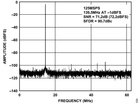
Figure 31. Single-Tone 16k FFT with f_{IN} = 139.5 MHz, f_{SAMPLE} = 125 MSPS
