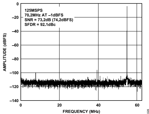
Figure 30. Single-Tone 16k FFT with f_{IN} = 70.2 MHz, f_{SAMPLE} = 125 MSPS
