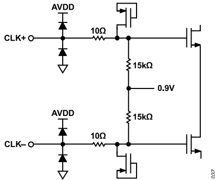
Figure 46. Equivalent Clock Input Circuit
