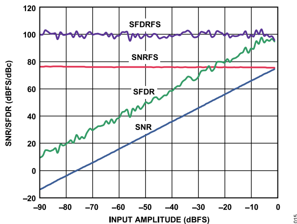
Figure 17. SNR/SFDR vs. Analog Input Level; f_{IN} = 9.7 MHz, f_{SAMPLE} = 80 MSPS
