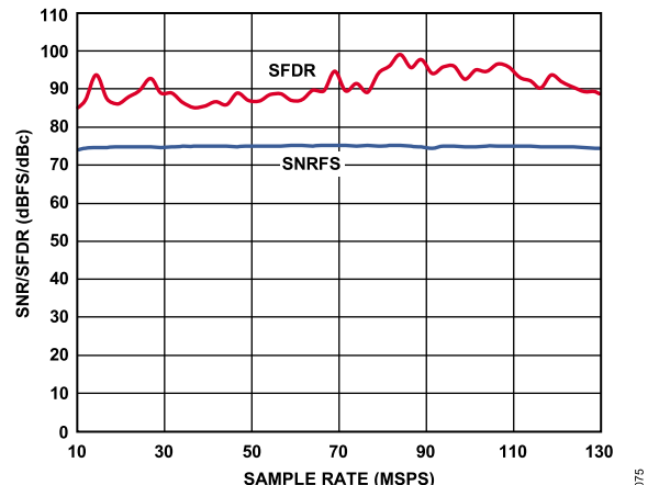
Figure 44. SNR/SFDR vs. Sample Rate; f_{IN} = 70 \text{ MHz} , f_{SAMPLE} = 125 \text{ MSPS}
