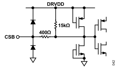
Figure 51. Equivalent CSB Input Circuit
