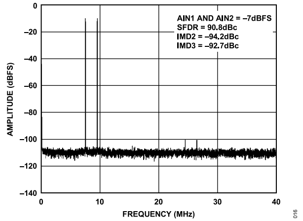
Figure 18. Two-Tone 16k FFT with f_{IN1} = 70.5 MHz and f_{IN2} = 72.5 MHz, f_{SAMPLE} = 80 MSPS
