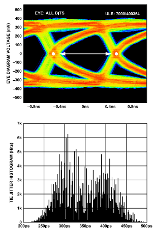
Figure 68. Data Eye for LVDS Outputs in ANSI-644 Mode with Trace Lengths of Less Than 24 Inches on Standard FR-4 Material, External 100 Ω Far-End Termination Only
