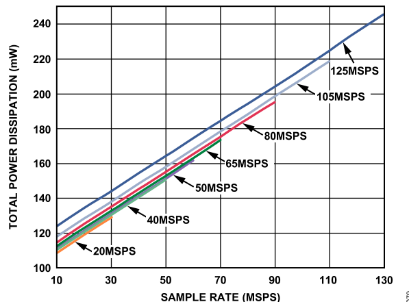
Figure 65. Total Power Dissipation vs. f_{\text{SAMPLE}} for f_{\text{IN}} = 9.7 \text{ MHz}
