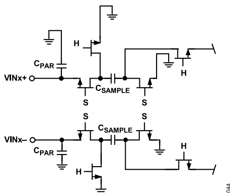
Figure 53. Switched-Capacitor Input Circuit
