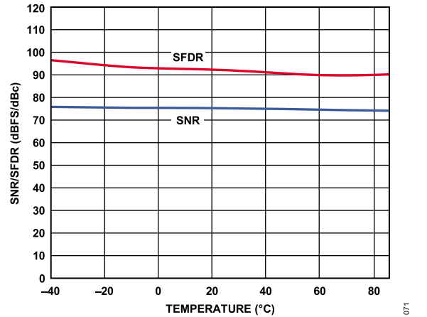
Figure 38. SNR/SFDR vs. Temperature; f_{IN} = 9.7 \text{ MHz} , f_{SAMPLE} = 125 \text{ MSPS}
