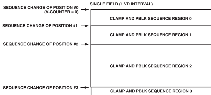
Figure 12. Clamp and Blanking Sequence Flexibility
