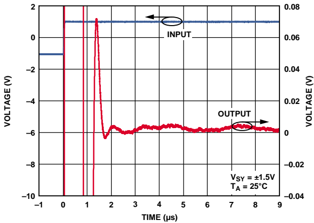
Figure 30. Settling Time
