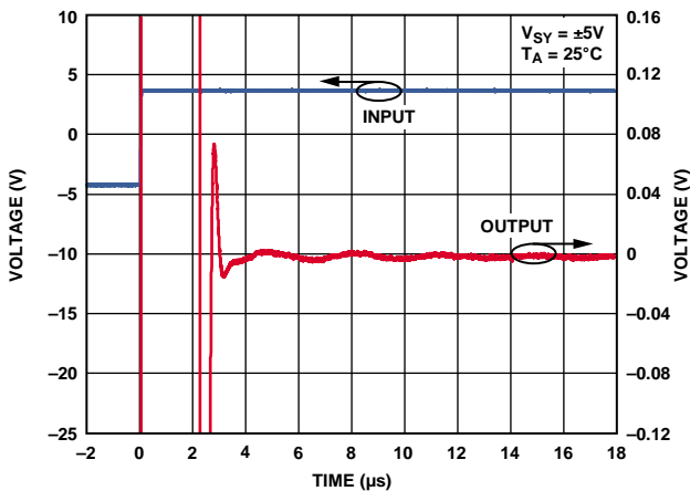
Figure 61. Settling Time
