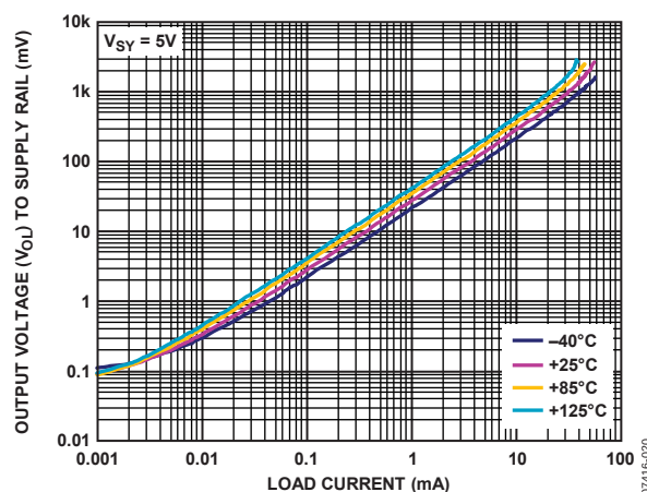
Figure 22. Output Voltage ( V_{OI} ) to Supply Rail vs. Load Current and Temperature
