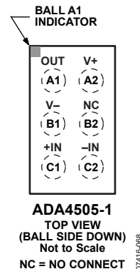
Figure 3. 6-Ball WLCSP (CB-6-7)
