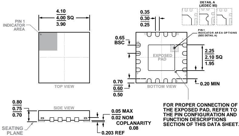
Figure 69. 16-Lead Lead Frame Chip Scale Package [LFCS] 4 mm x 4 mm Body and 0.75 mm Package Height (CP-16-23) Dimensions shown in millimeters
