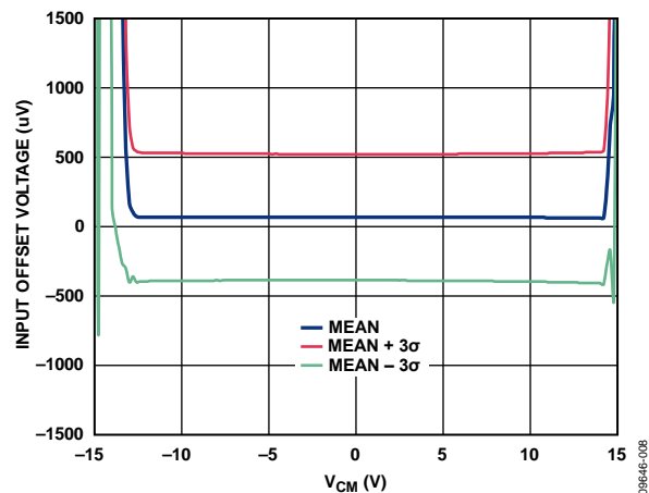
Figure 14. Input Offset Voltage vs. Input Common-Mode Voltage (V CM ), V SY = ±15 V, R L = ∞
