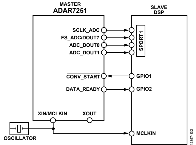
Figure 40. ADC Serial Master Mode with CONV_START
