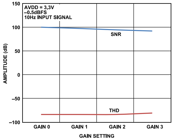
Figure 48. SNR and THD Across Gain Settings
