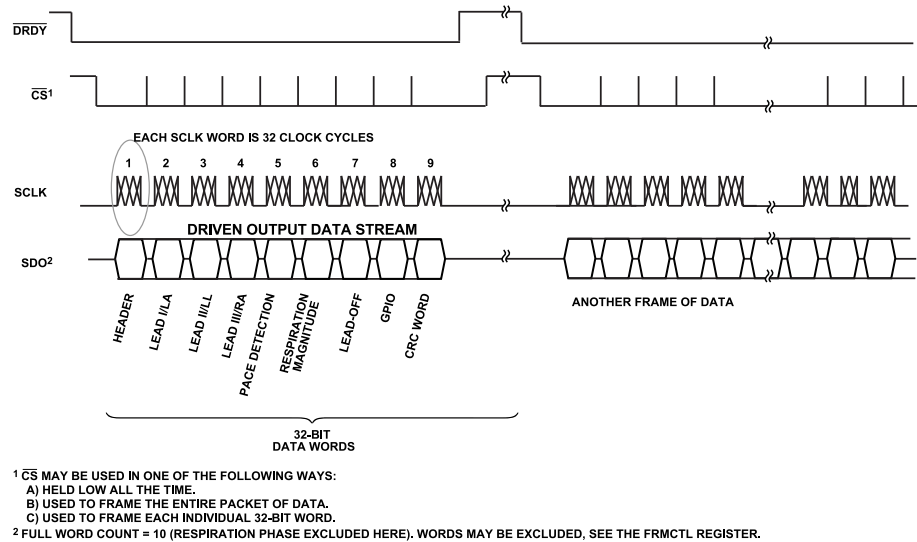
Figure 79. Output Frame Structure for 2 kHz and 16 kHz Data Rates with SDO Data Configured for Electrode or Lead Data
