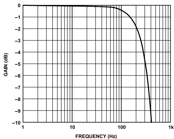
Figure 24. Filter Response with 250 Hz Filter Enabled, 2 kHz Data Rate; See Figure 72 for Digital Filter Overview
