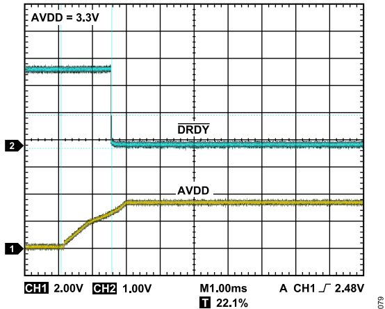
Figure 49. Power Up AVDD Line to \overline{\text{DRDY}} Going Low (Ready)
