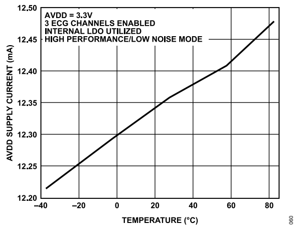
Figure 30. Typical AVDD Supply Current vs. Temperature, Using Internal ADVCD/DVDD Supplies
