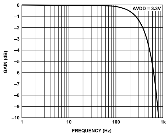
Figure 25. Filter Response with 450 Hz Filter Enabled, 2 kHz Data Rate; See Figure 72 for Digital Filter Overview
