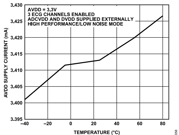
Figure 31. Typical AVDD Supply Current vs. Temperature, Using Externally Supplied ADVCD/DVDD
