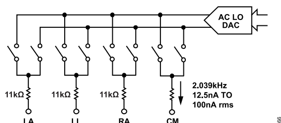
Figure 66. Simplified AC Lead-Off Configuration
