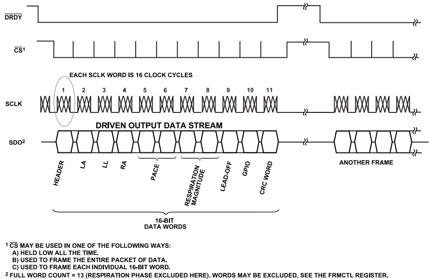
Figure 80. Output Frame Structure for 128 kHz Data Rate with SDO Data Configured for Electrode Data (The 128 kHz Data Rate Can Provide Single-Ended Electrode Data or Analog Lead Mode Data Only. Digital Lead Mode Is Not Available at 128 kHz Data Rate.)
