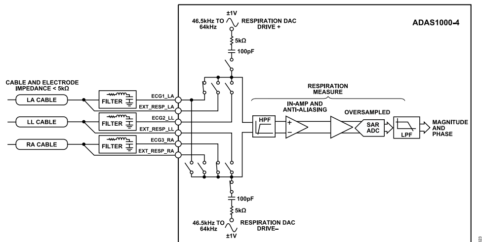
Figure 67. Simplified Respiration Block Diagram
