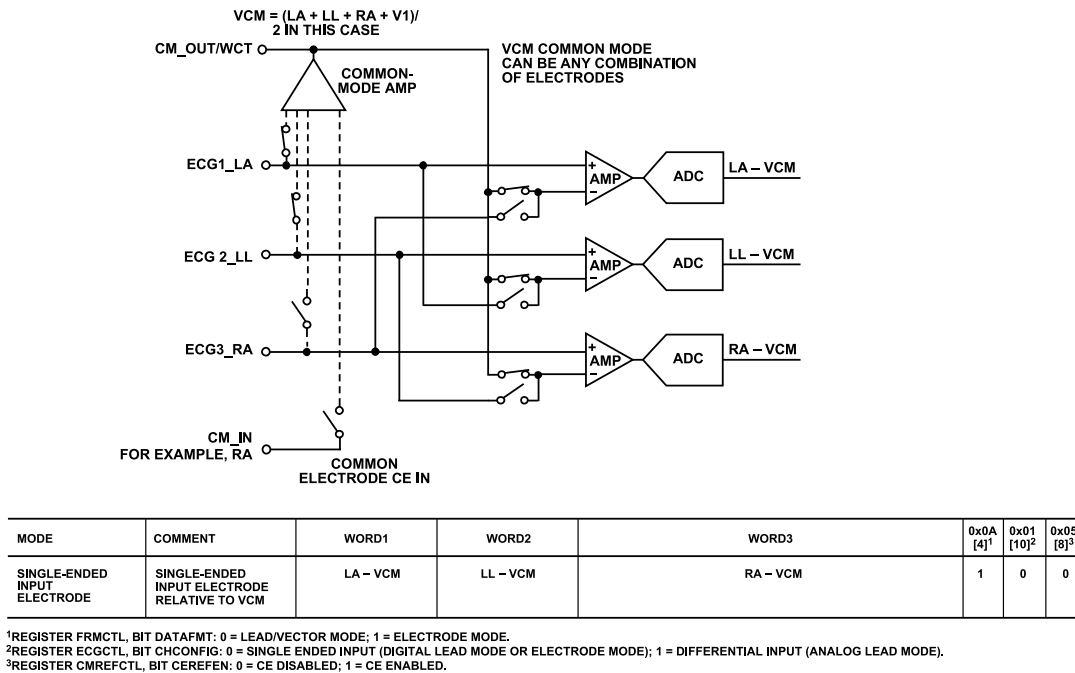
Figure 59. Electrode and Lead Configurations, Single-Ended Input Electrode
