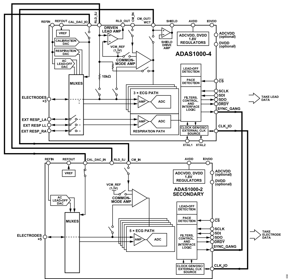
Figure 74. Configuring Multiple Devices to Extend Number of Electrodes/Leads (This Example Uses ADAS1000-4 as a Primary Device and ADAS1000-2 as a Secondary Device; Other Arrangements Possible)
