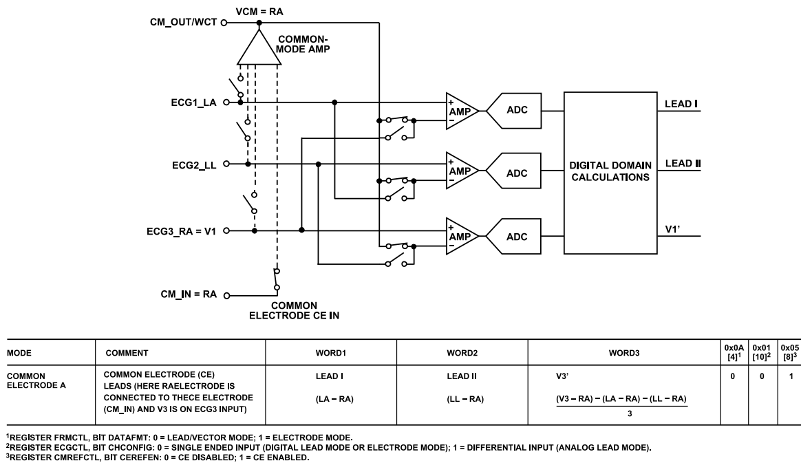
Figure 58. Electrode and Lead Configurations, Common Electrode A
