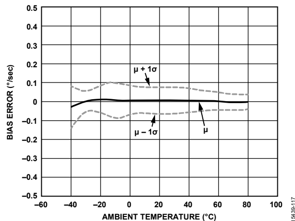
Figure 17. ADIS16467-3 Gyroscope Bias Error vs. Ambient Temperature
