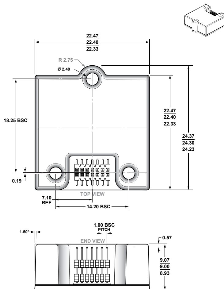
Figure 55. 14-Lead Module with Connector Interface [MODULE] (ML-14-6)
