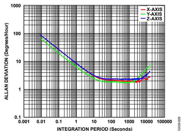
Figure 9. Gyroscope Allan Deviation, T_c = 25^\circ\text{C} , ADIS16467-2
