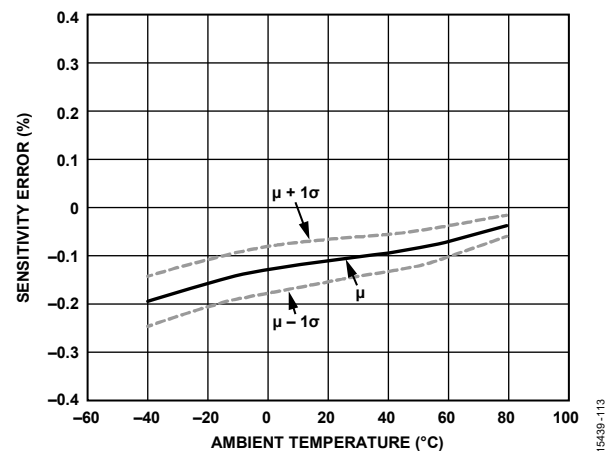
Figure 13. ADIS16467-2 Gyroscope Sensitivity Error vs. Ambient Temperature
