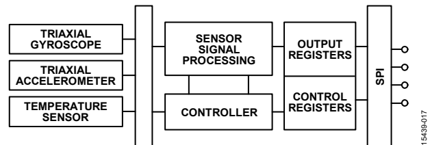
Figure 25. Basic Operation of the ADIS16467
