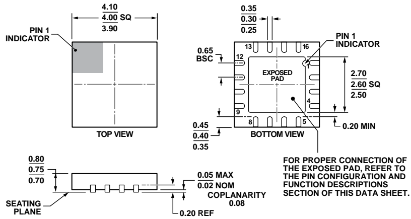
Figure 41. 16-Lead Lead Frame Chip Scale Package [LFCSP_WQ] 4 mm x 4 mm Body, Very Very Thin Quad (CP-16-17)
