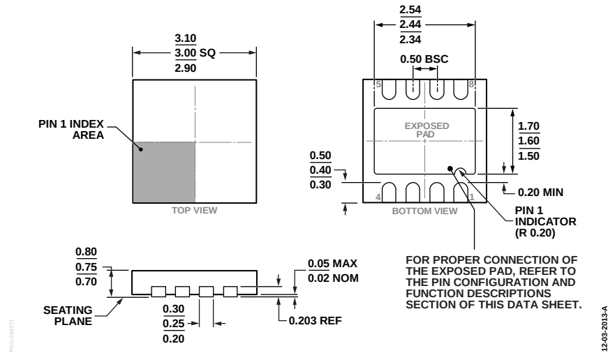
Figure 65. 8-Lead Lead Frame Chip Scale Package [LFCSP_WD] 3 mm × 3 mm Body, Very Very Thin, Dual Lead (CP-8-21) Dimensions shown in millimeters
