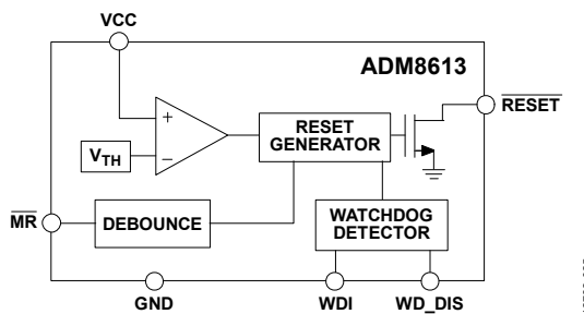
Figure 25. ADM8613 Functional Block Diagram
