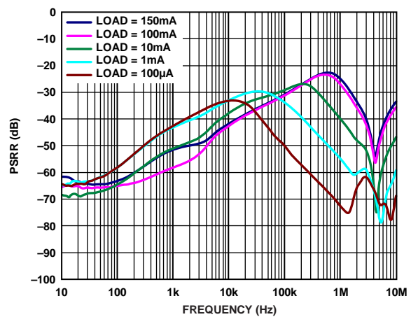
Figure 20. PSRR vs. Frequency, Various Load Currents, V_{OUT} = 2.5 V , V_{IN} = 3.5 V
