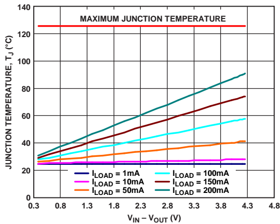
Figure 51. 500 mm 2 of PCB Copper, LFCSPT, T A = 25°C
