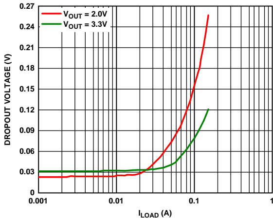
Figure 16. Dropout Voltage vs. Load Current ( I_{LOAD} )
