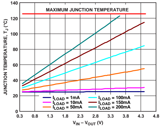
Figure 52. 100 mm 2 of PCB Copper, LFCSPT, T A = 25°C
