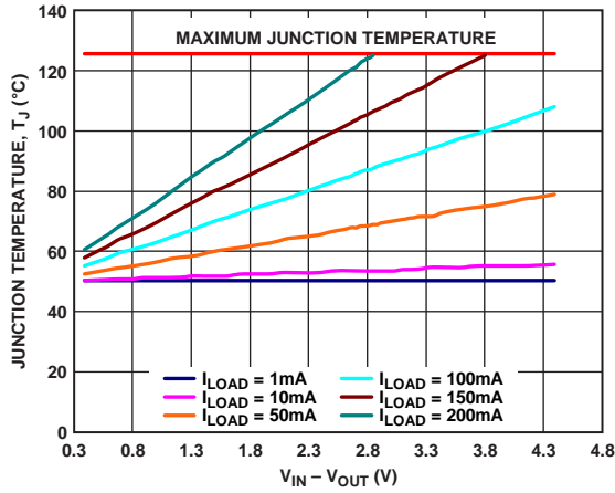
Figure 49. 500 mm 2 of PCB Copper, TSOT, T A = 50°C
