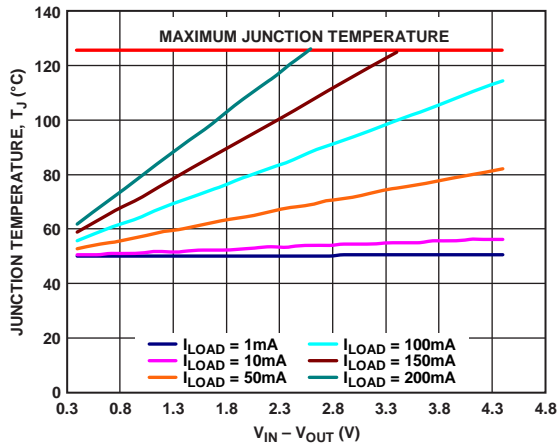
Figure 50. 100 mm 2 of PCB Copper, TSOT, T A = 50°C
