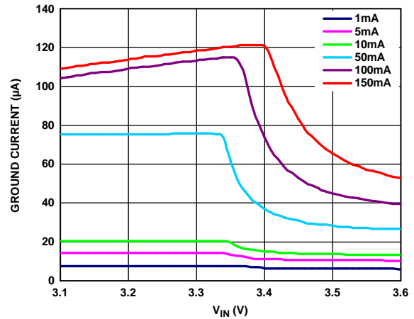
Figure 18. Ground Current vs. Input Voltage ( V_{IN} ) in Dropout
