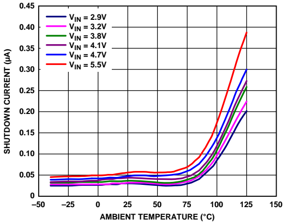
Figure 15. Shutdown Current vs. Ambient Temperature at Various Input Voltages
