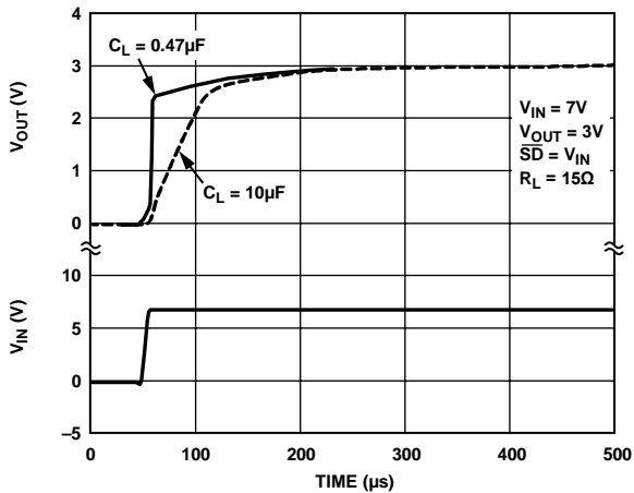
Figure 12. Power-Up Response
