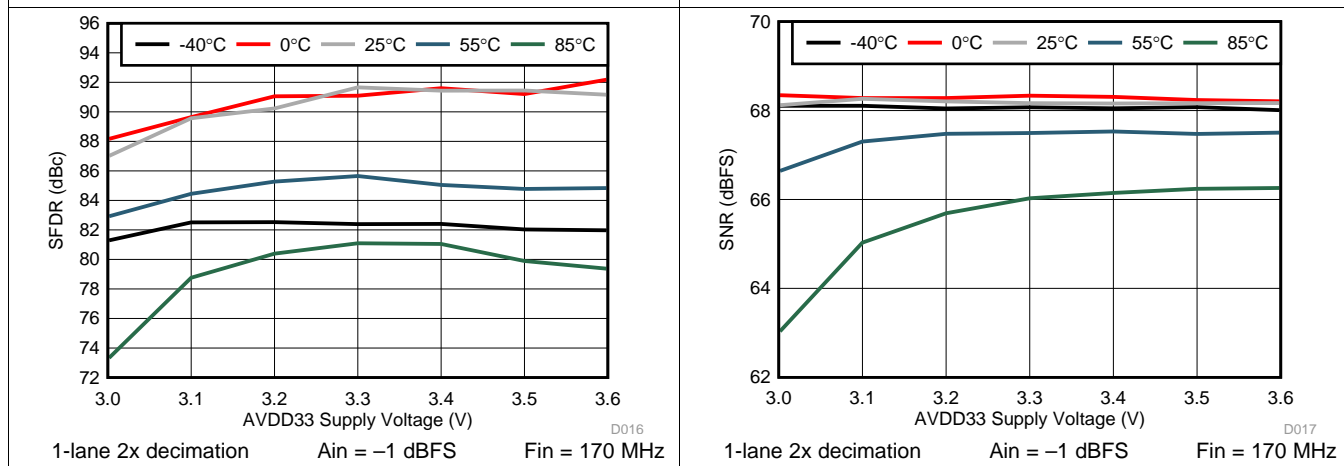
Figure 20. SFDR vs. AVDD33
