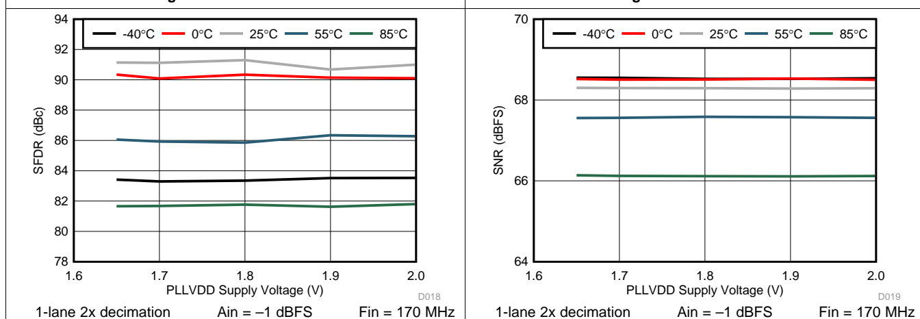
Figure 22. SFDR vs. PLLVDD
