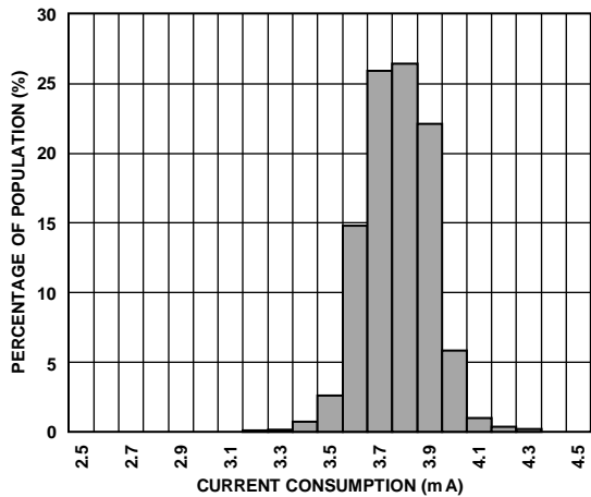
Figure 12. Current Consumption at 25°C ( V_{RATIO} = 5 V )
