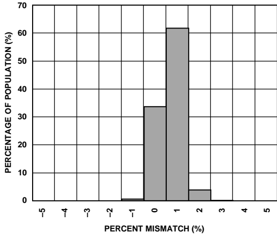
Figure 10. Self-Test Mismatch at 25°C ( V_{RATIO} = 5 V )
