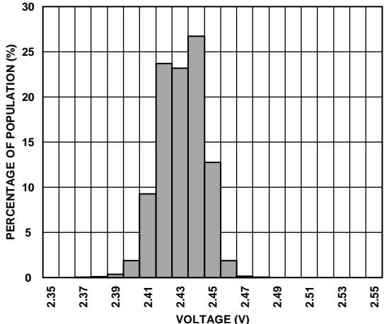
Figure 13. V_{TEMP} Output at 25°C ( V_{RATIO} = 5 V )
