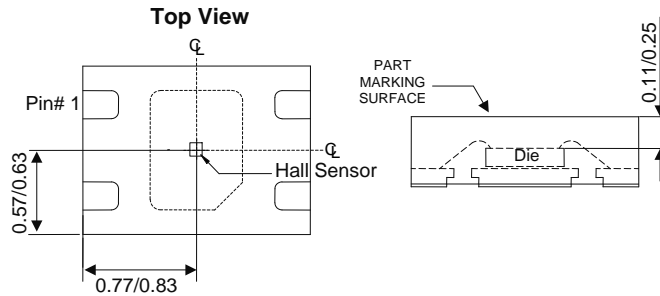
Sensor Location
