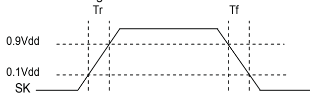
Figure 8.4 Rise time and fall time
