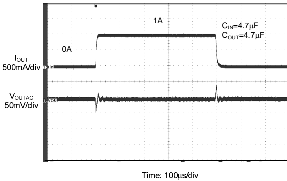
Figure 46. Load Transient
