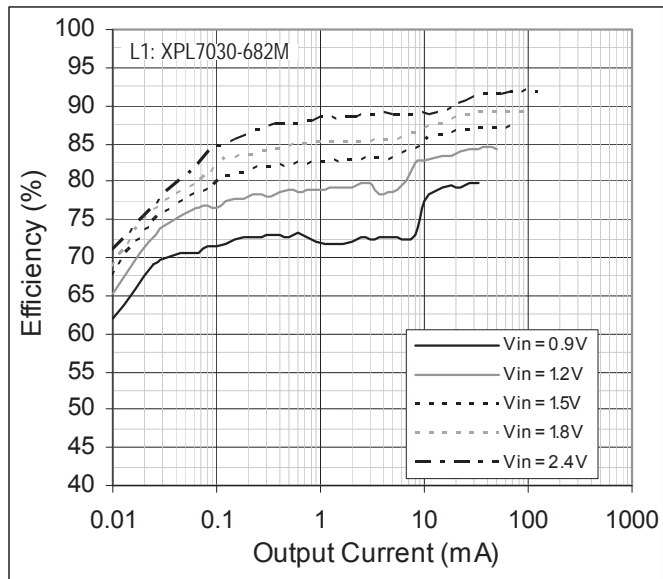
Figure 10: Efficiency vs. Output Current; V_{OUT} = 3.0V
