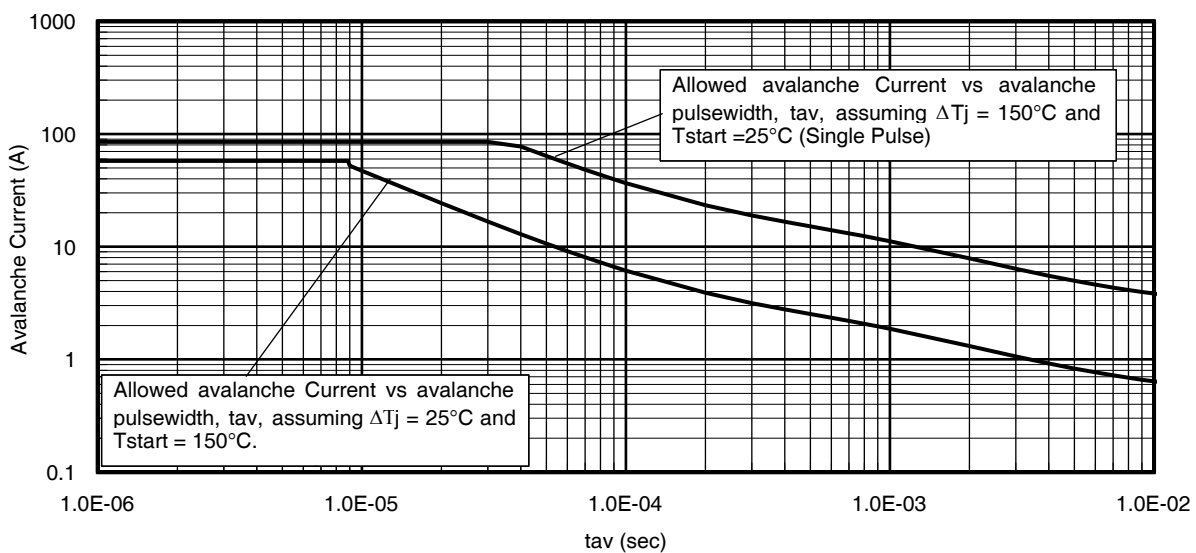
Fig 16. Single Avalanche Event: Pulse Current vs. Pulse Width
