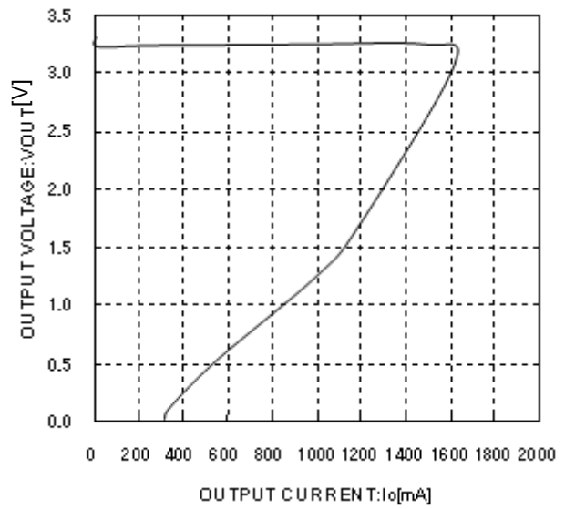
Fig.4 Load Stability
