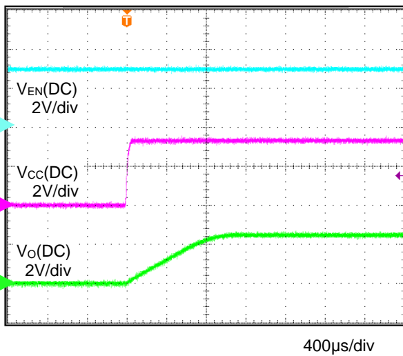
Figure 10. Input sequence 1 (Vcc:0V to 3.3V) (C IN =C OUT =1µF, Ta=-40°C, tr=30µs)
