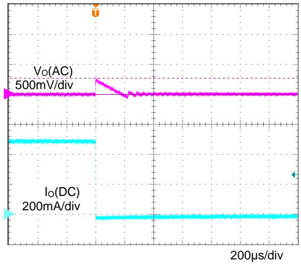
Figure 9. Transient Response (Io:500mA to 1mA) (C IN =C OUT =1µF, Ta=+105°C)
