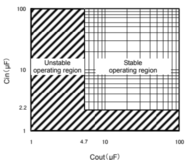
C in vs C out 1.0V ≤ V O < 3.0V (Reference data)
