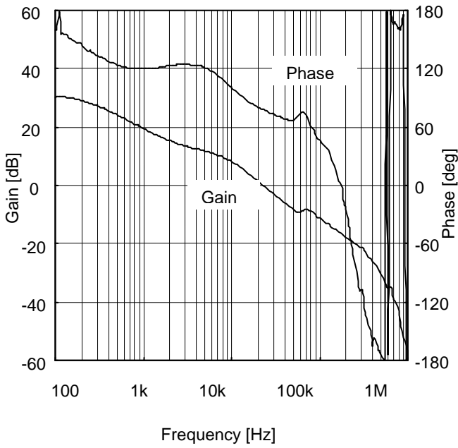
Figure 27. Frequency Response Property 1 ( V_{CC} = 3.0V , I_O = 200\text{ mA} )
