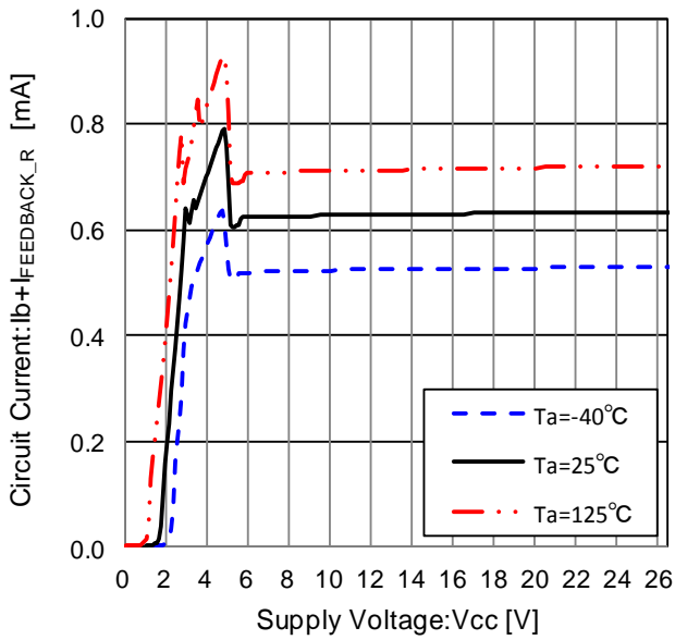
Figure 11. Circuit Current ( I_{FEEDBACK\_R}^{(Note\ 1)} \approx 75\mu\text{A} )
