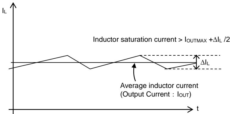
Figure 62. Waveform of Current through Inductor
