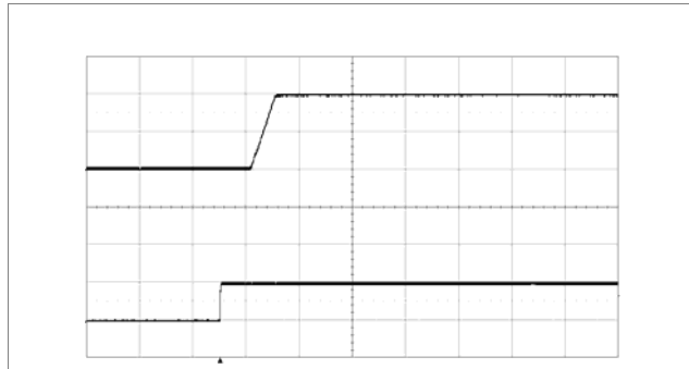
Start-up by enabling CTRL signal at: T_{P1} = +25\text{ }^\circ\text{C} , V_I = 12\text{ V} , V_O = 1.0\text{ V} C_O = 470\text{ }\mu\text{F}/10\text{ m}\Omega , I_O = 40\text{ A} Top trace: output voltage (0.5 V/div.). Bottom trace: CTRL signal (5 V/div.). Time scale: (20 ms/div.).
