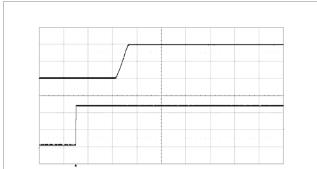
Start-up enabled by connecting V_I at: T_{P1} = +25\text{ }^\circ\text{C} , V_I = 12\text{ V} , V_O = 1.0\text{ V} C_O = 470\text{ }\mu\text{F}/10\text{ m}\Omega , I_O = 40\text{ A} Top trace: output voltage (0.5 V/div.). Bottom trace: input voltage (5 V/div.). Time scale: (20 ms/div.).
