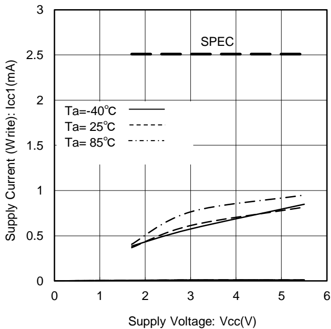
Figure 10. Supply Current (Write) vs Supply Voltage (fscI=400kHz)
