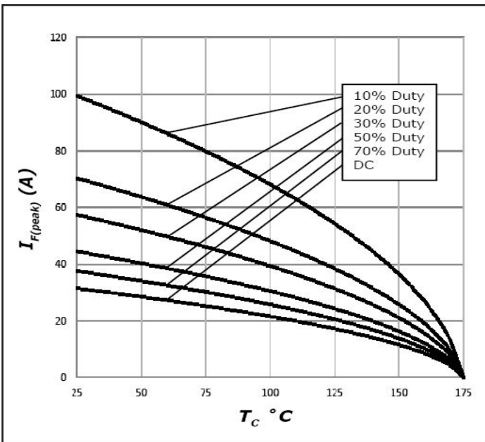
Figure 3. Current Derating
