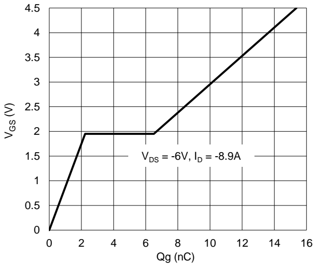
Figure 23. Gate Charge
