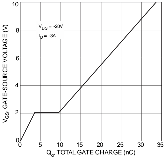
Figure 22 Gate-Charge Characteristics
