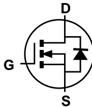
Internal Schematic
