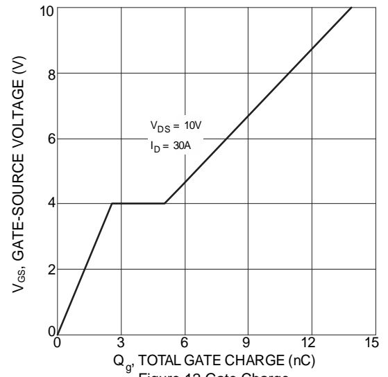
Figure 12 Gate Charge
