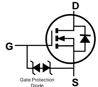
Equivalent Circuit
