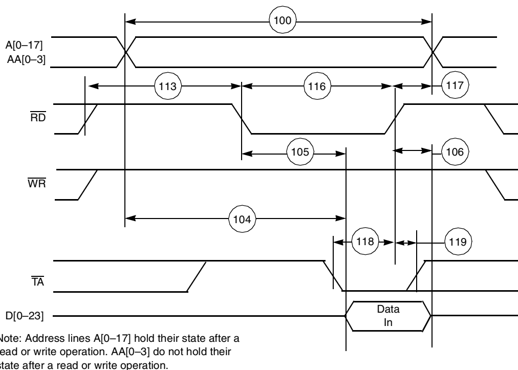
Figure 2-10. SRAM Read Access
