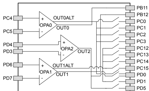
Figure 5.16. Opamp Pinout
