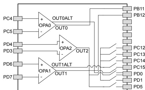
Figure 5.34. Opamp Pinout
