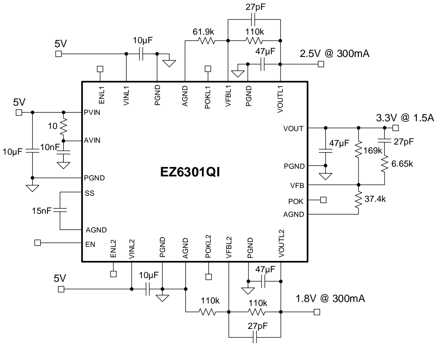
Figure 8: Application Schematic for V_{OUT} = 3.3\text{V} , V_{OUTL1} = 2.5\text{V} , V_{OUTL2} = 1.8\text{V}
