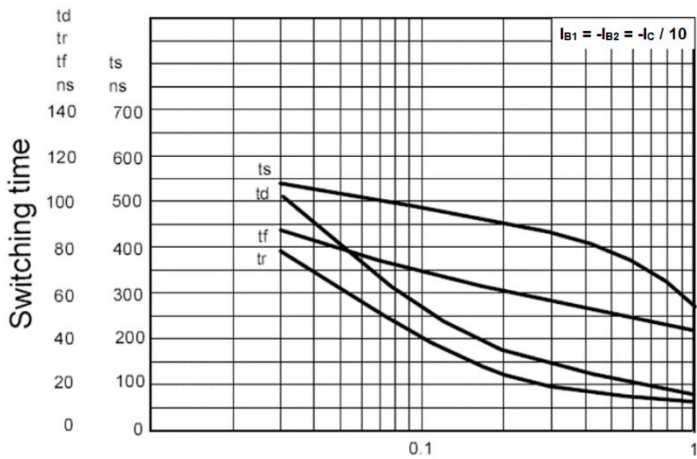
Switching Speeds
