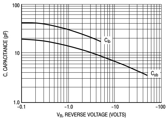
Figure 16. Capacitances
