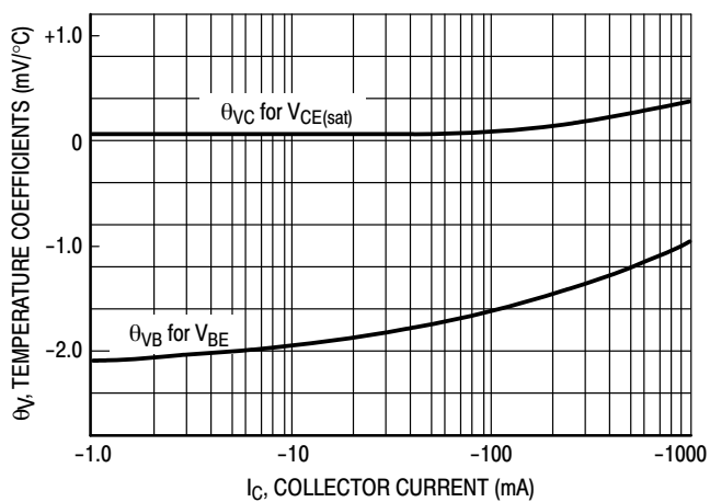
Figure 15. Temperature Coefficients
