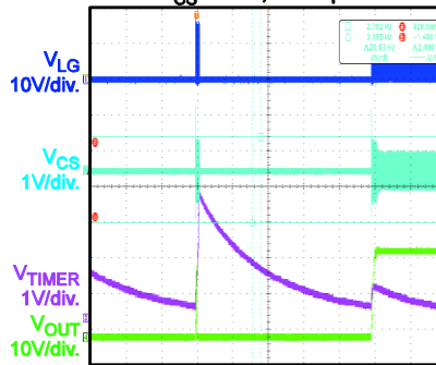
Over-Current Protection Recovery 0.8V < V_{CS} < 1.5V , Hiccup and Auto-Recovery
