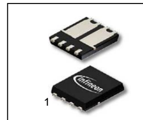
PG-TDSON-8
