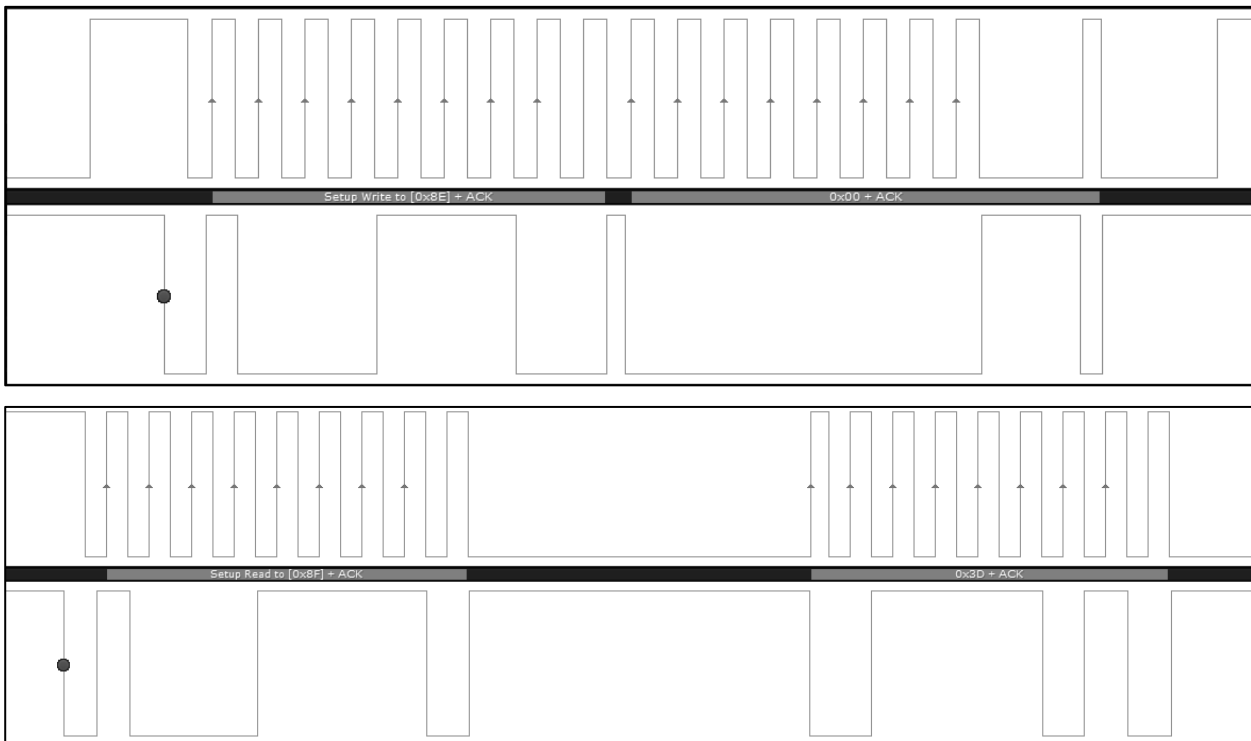
Figure 6-1 Typical polling example of IQS211A. The sequence addresses register 0x00 (top) and reads data (0x3D) from register 0x00 (bottom)
