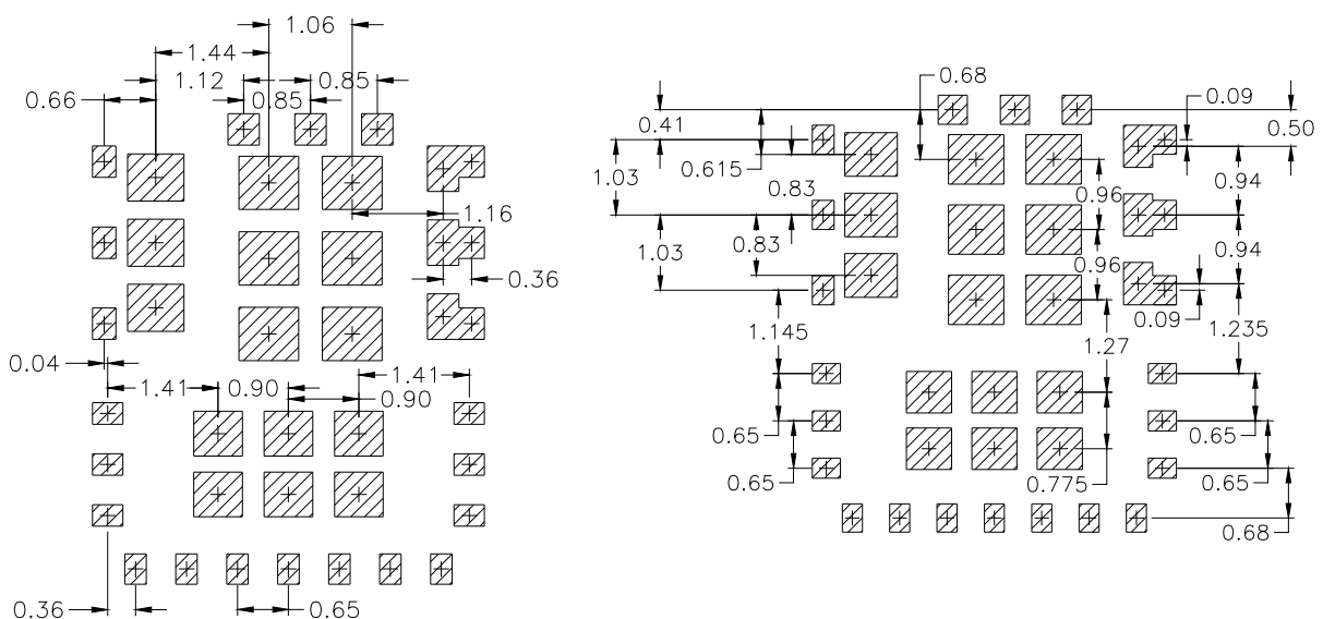
Stencil pad sizing (all dimensions in mm)
